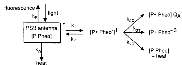
Fig. 2. Simplified scheme of energy conversion in PSII according to the reversible radical pair model, featuring rapid excitation equilibration between the PSII antenna and the reaction center chlorophyll P ( P_{680} ). Excitation trapping (rate constant k_1 ), which results in the primary radical pair [P^+Pheo^-]^1 in the singlet state, is assumed to be reversible ( k_{-1} ). Three further reactions of the primary radical pair are considered: k_{2Q} , photochemical energy conversion by electron transfer to Q_A ; k_{2T} , spin dephasing resulting in triplet state of radical pair; k_{2D} , nonradiative decay to ground state. Fluorescence yield (rate constant k_F ) reflects excitation density in PSII (antenna, including P), which is determined by light absorption, primary radical pair recombination ( k_{-1} ) and competing non-radiative decay ( k_D ). Variable fluorescence is defined as the increase in fluorescence yield when the primary stable acceptor, Q_A , is reduced. It is considered to be caused by a decrease in k_1 and an increase in k_{-1} , and to be modulated by k_D , k_{2T} and k_{2D} . See text for further explanations.
